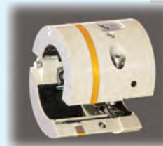
Split and cover-up system
